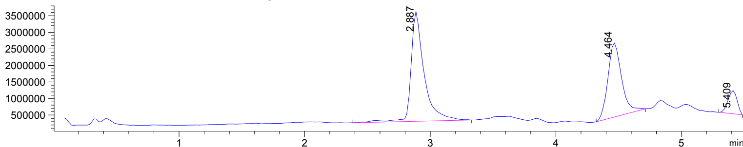
Integration Results for DAD1 A, Sig=254,4 Ref=off
